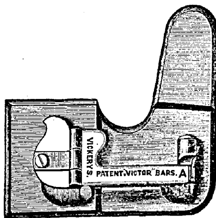
Рис. 515. „Vickery's safety saddle bar“.
